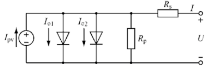
Fig. 2. Double diode equivalent circuit model of a photovoltaic cell in a photovoltaic array.
